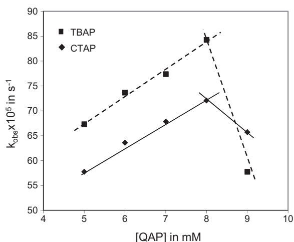
Fig. 3. Variation of [QAP] in mM with rate constants of self-oxidation/dissociation at a fixed \beta -CD concentration of 9.0 mM in aqueous medium at 22.0 \pm 1^\circ\text{C} .
