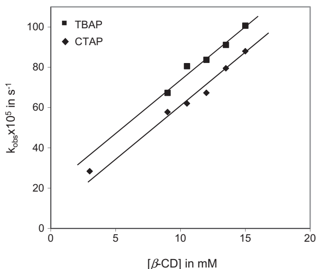
Fig. 2. Variation of [\beta\text{-CD}] in mM with rate constants of self-oxidation/dissociation of QAPs in aqueous medium at 22.0 \pm 1^\circ\text{C} .
