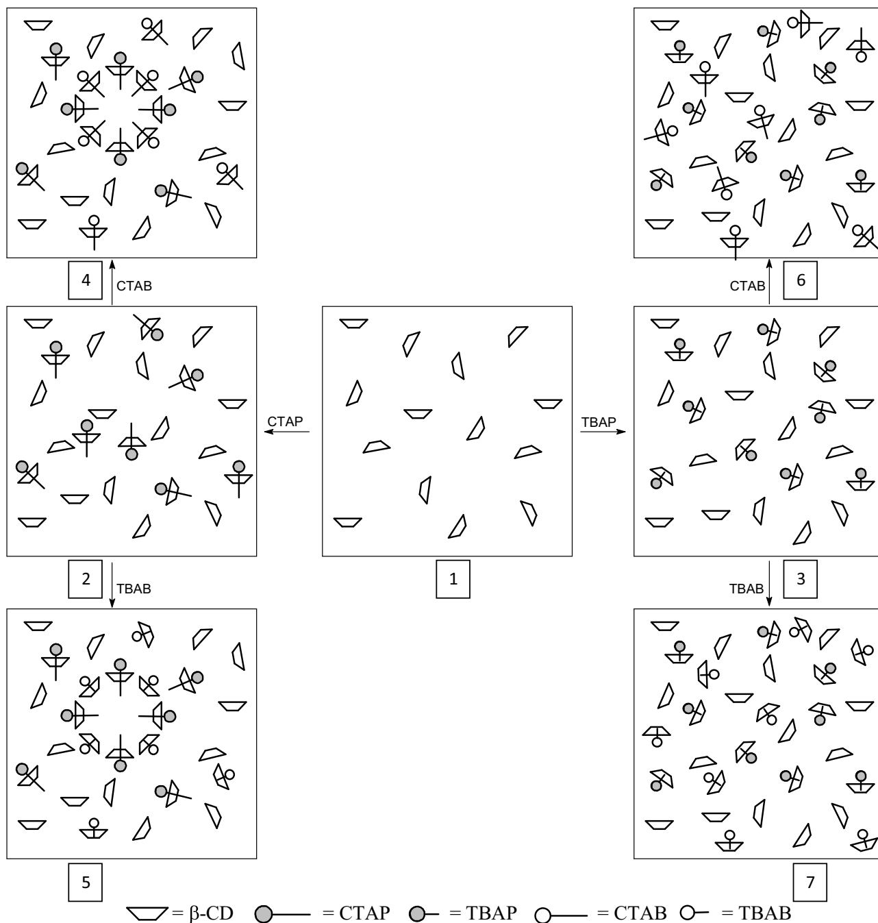
Scheme 2. Impact of CTAB and TBAB on CTAP and TBAP dissolved in \beta -CD aqueous phase (1: \beta -CD aqueous phase, 2: CTAP dissolved in \beta -CD aqueous phase, 3: TBAB dissolved in \beta -CD aqueous phase, 4: partitioning of CTAP to CTAB micellar submicro phase, 5: partitioning of CTAP to CTAB-TBAB micellar submicro phase, 6: CTAB-enhanced inclusion complexation of TBAB, 7: TBAB-enhanced inclusion complexation of CTAP).
