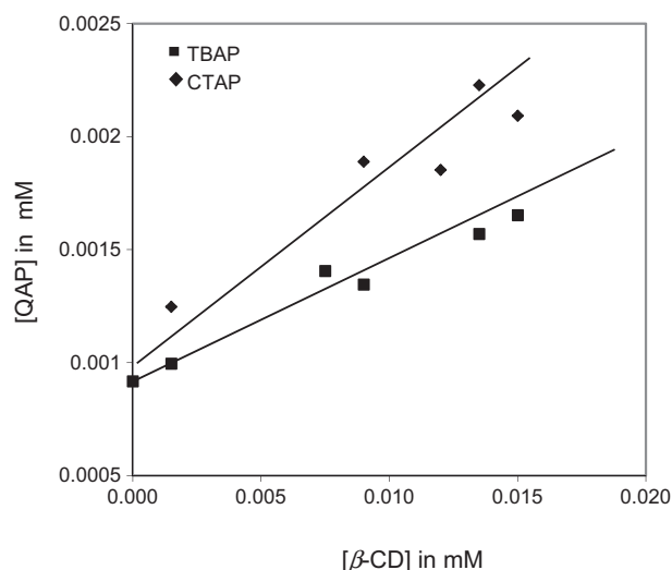
Fig. 1. Variation of [\beta\text{-CD}] in mM with [\text{QAP}] in mM in aqueous medium at 22.0 \pm 1^\circ\text{C} .
