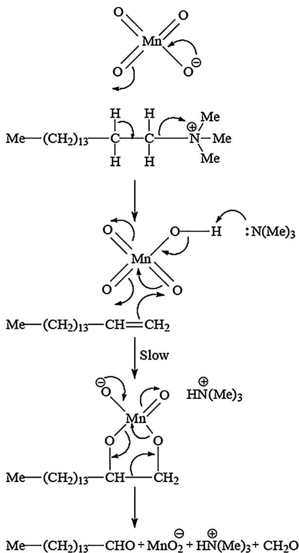
Scheme 1. Self-oxidation of CTAP in chloroform medium.
