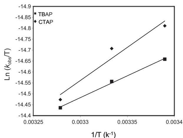
Fig. 5. Plot of \ln(k_{\text{obs}}/T) versus 1/T at a fixed \beta -CD concentration of 9.0 mM in aqueous medium.
